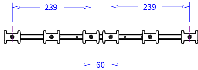
30-er truss
